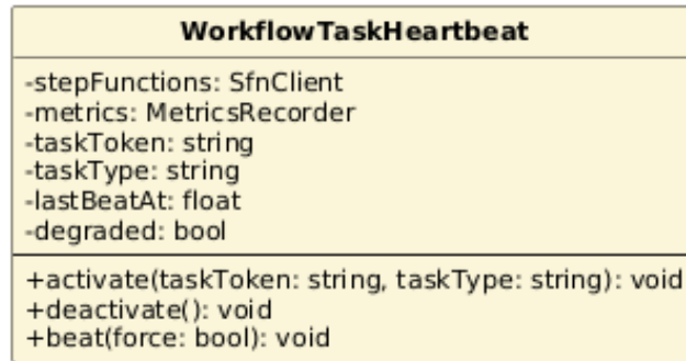
Figura 78: Classe — WorkflowTaskHeartbeat
