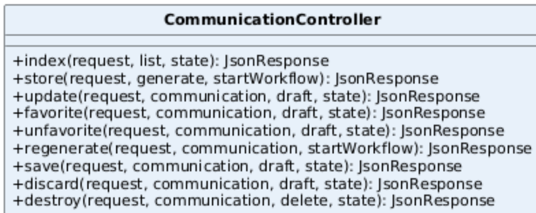
Figura 47: Classe — CommunicationController
