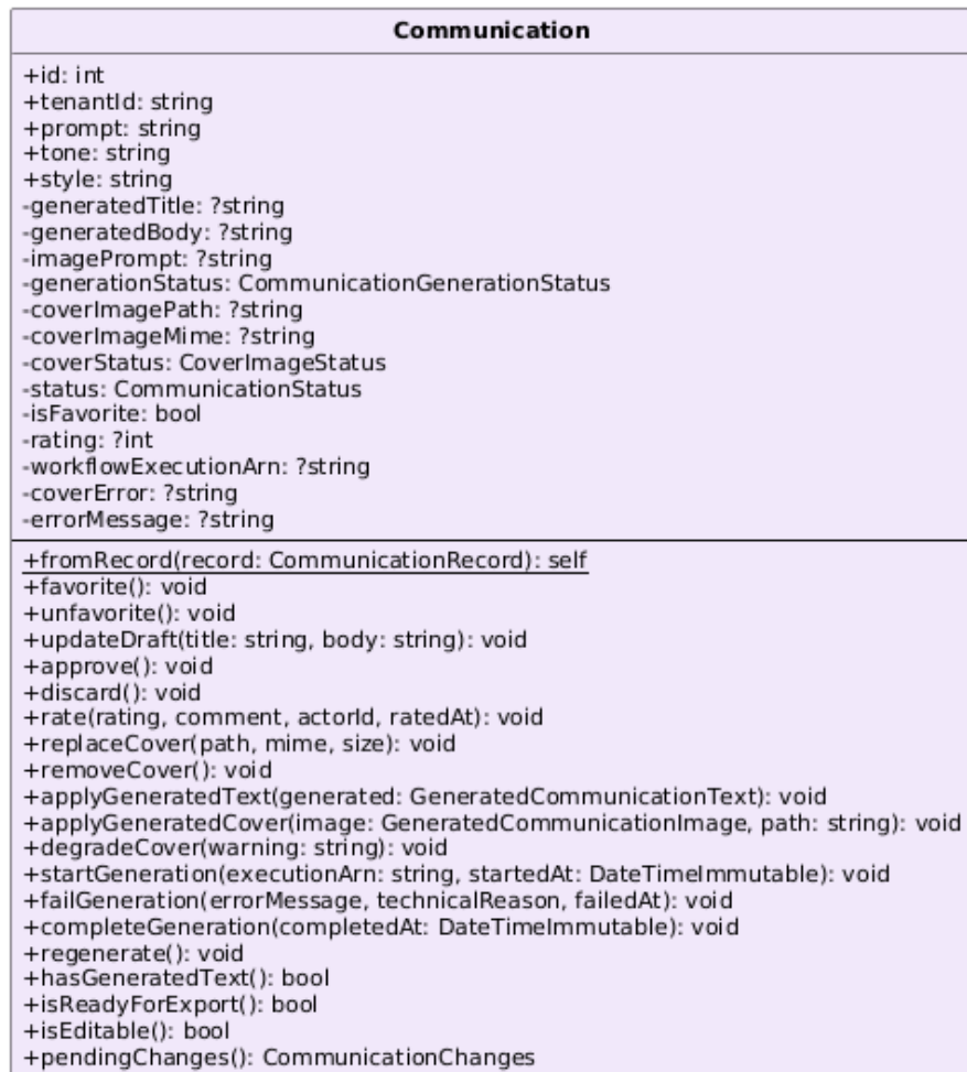
Figura 53: Classe — Communication
