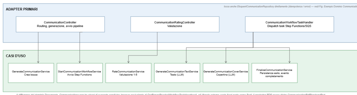
Figura 5: Component Diagram — Modulo Communications
