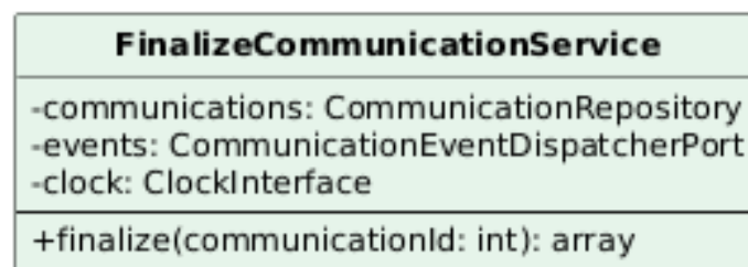
Figura 58: Classe — FinalizeCommunicationService
