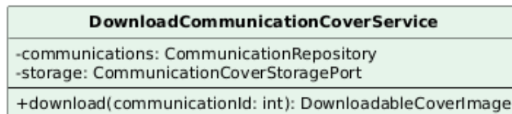
Figura 63: Classe — DownloadCommunicationCoverService
