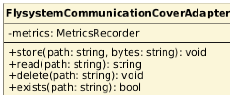
Figura 72: Classe — FlysystemCommunicationCoverAdapter
