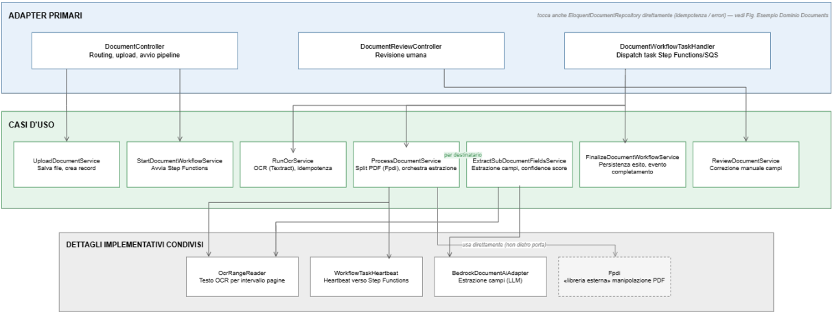
Figura 4: Component Diagram — Modulo Documents
