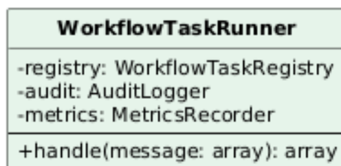
Figura 76: Classe — WorkflowTaskRunner
