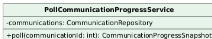
Figura 59: Classe — PollCommunicationProgressService
